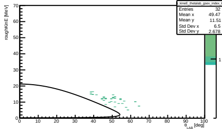
h_kineE_thetalab_gsex_z_600--700
