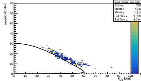
h_kineE_gsex_thetalab_z_others
