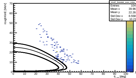
h_kineE_thetalab_exex_z_500--600
