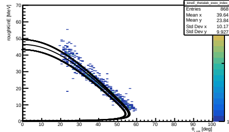
h_kineE_thetalab_exex_z_200--300
