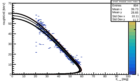
h_kineE_thetalab_exex_z_0--100
