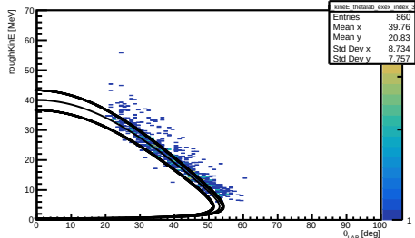
h_kineE_thetalab_exex_z_300--400
