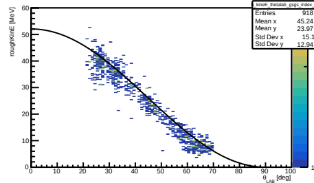
h_kineE_thetalab_gsgs_z_500--600
