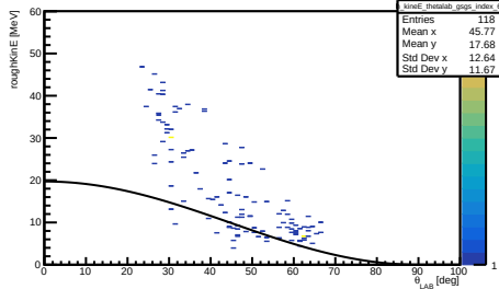
h_kineE_thetalab_gsgs_z_600--700
