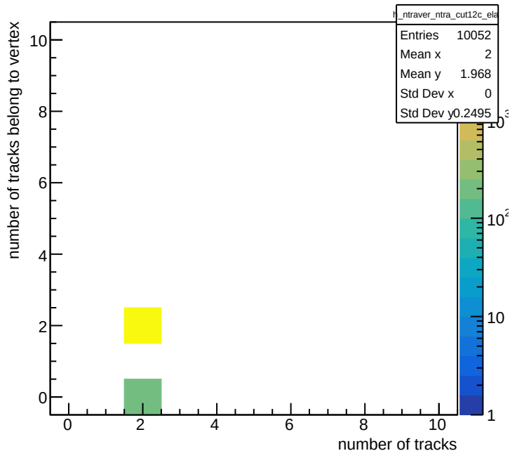
tracks with vertex ( \phi_1 - \phi_2 - 180 < 10 , track == 2, 12c12c)
