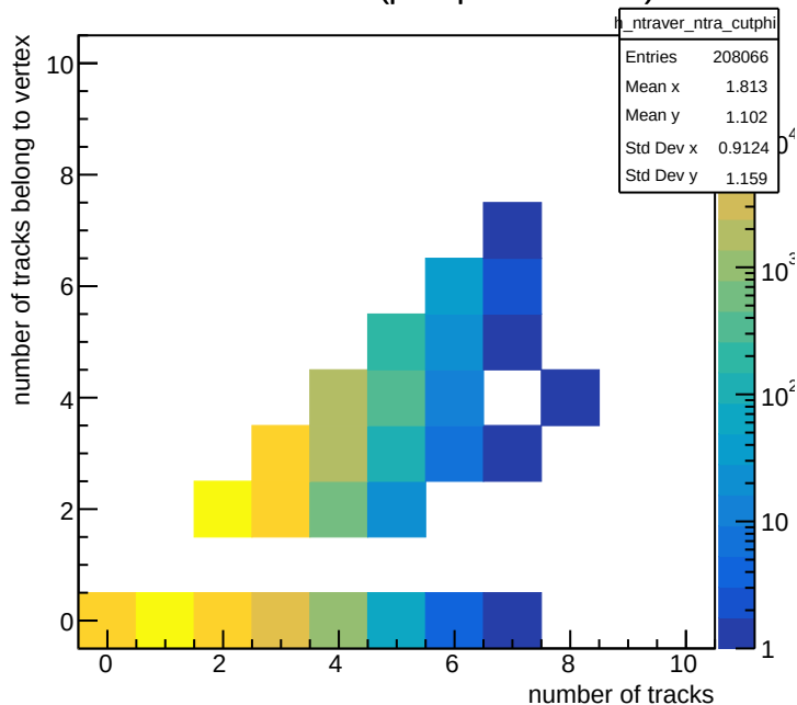
tracks with vertex ( \phi_1 - \phi_2 - 180 < 10 )
