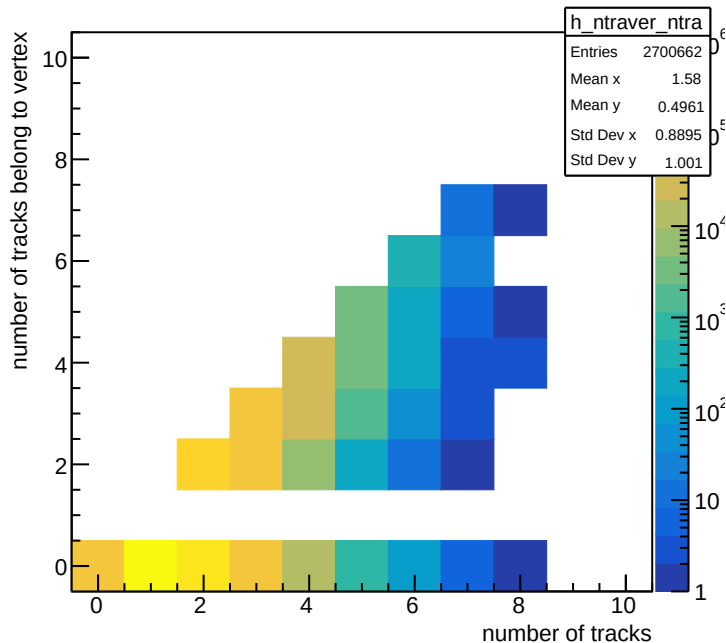
tracks with vertex
