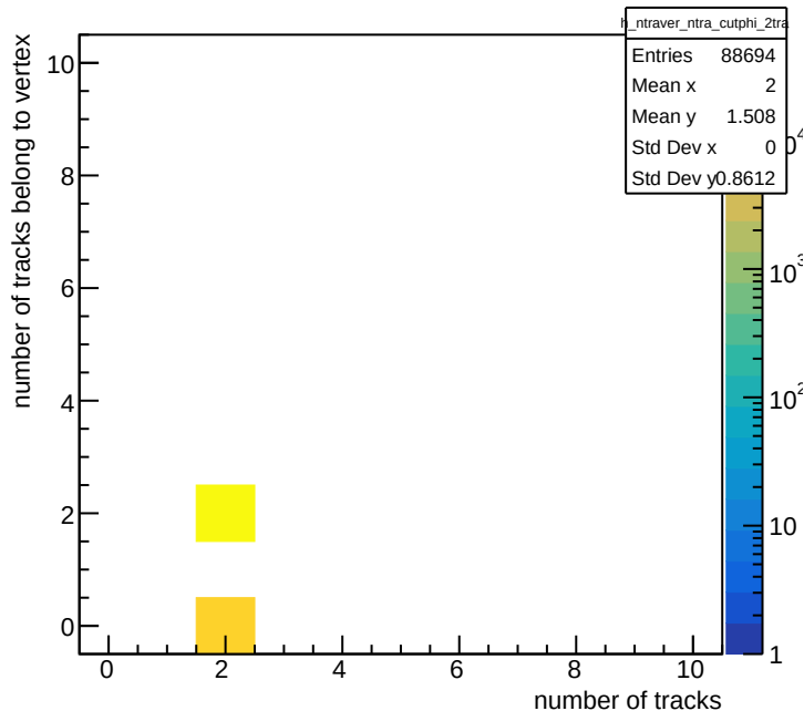
tracks with vertex ( \phi_1 - \phi_2 - 180 < 10 , track == 2)
