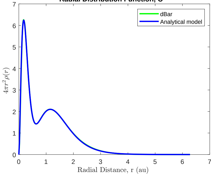
Radial Distribution Function, C^{+1}
