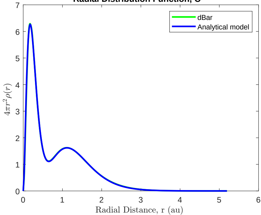
Radial Distribution Function, C^{+2}
