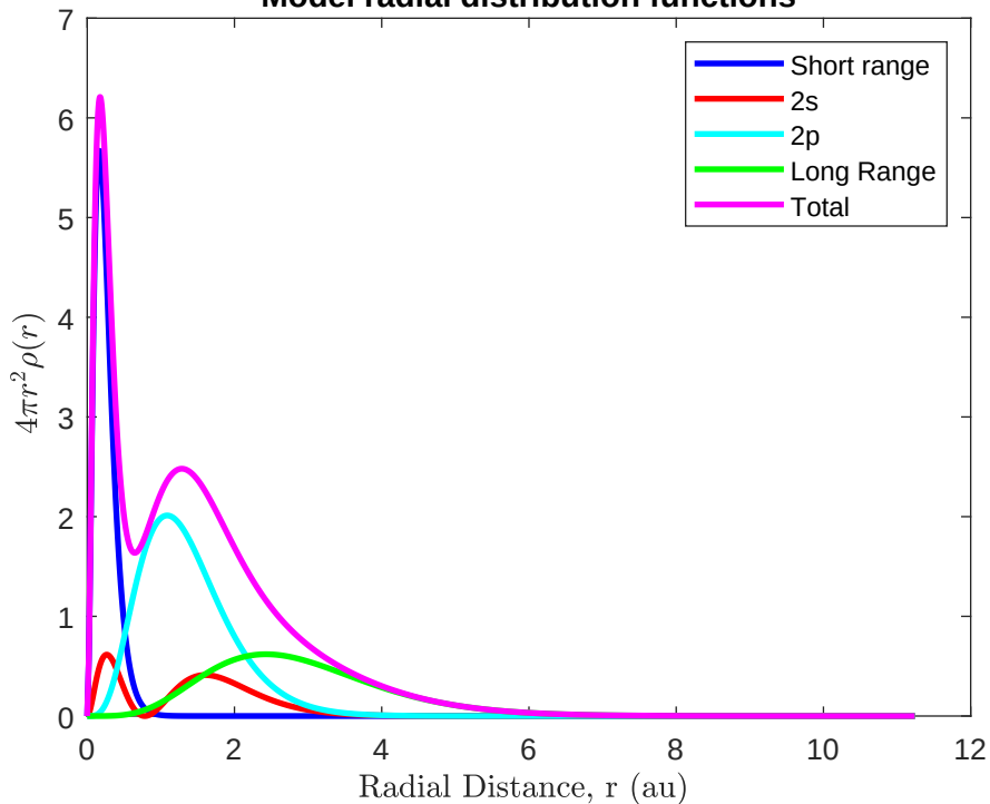
Model radial distribution functions
