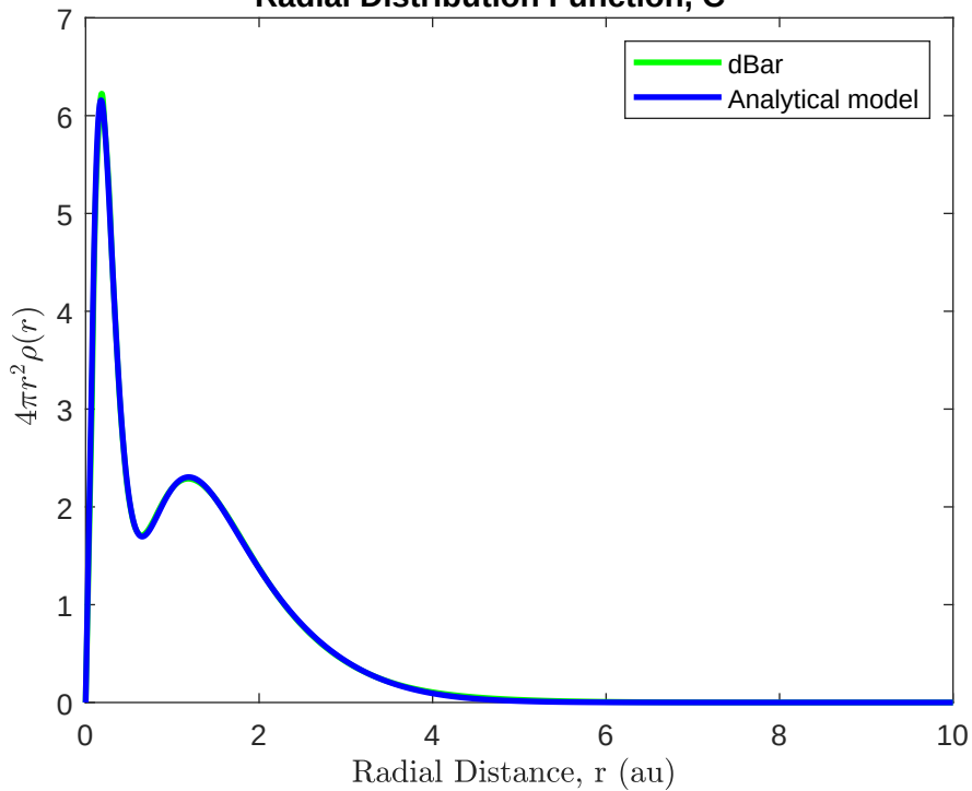
Radial Distribution Function, C^{\text{exc1}}
