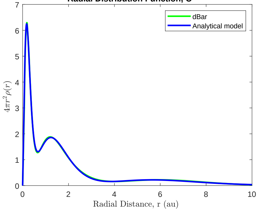
Radial Distribution Function, C^{\text{exc3}}
