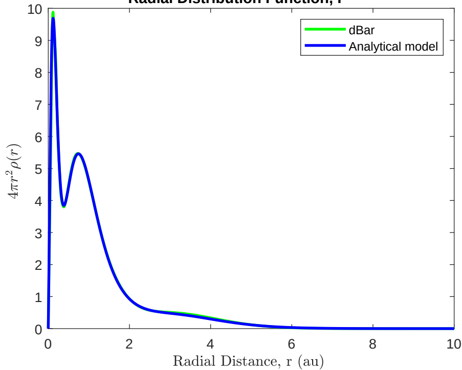
Radial Distribution Function, F^{\text{exc1}}
