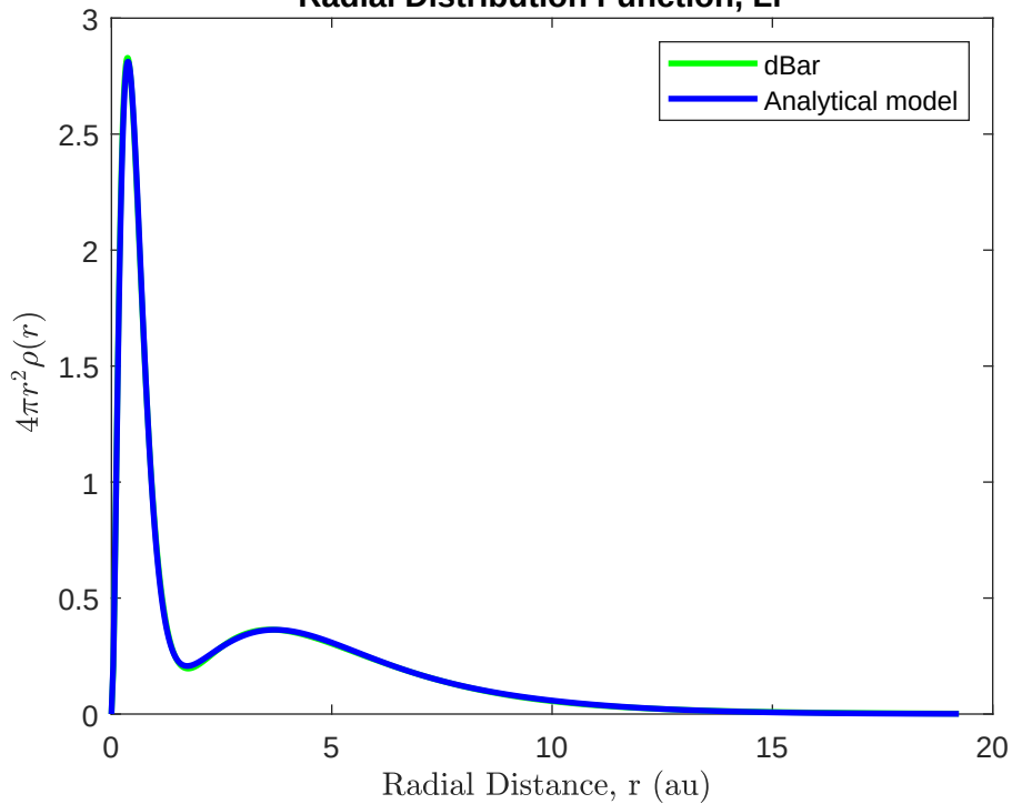
Radial Distribution Function, \text{Li}^{-1}
