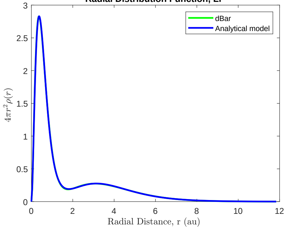
Radial Distribution Function, \text{Li}^0
