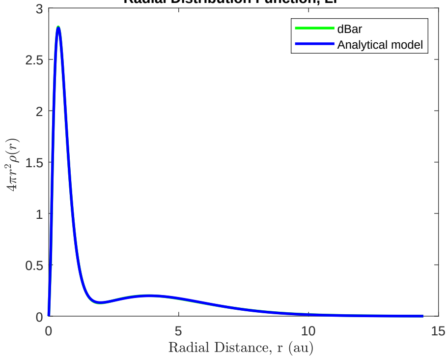
Radial Distribution Function, \text{Li}^{\text{exc1}}
