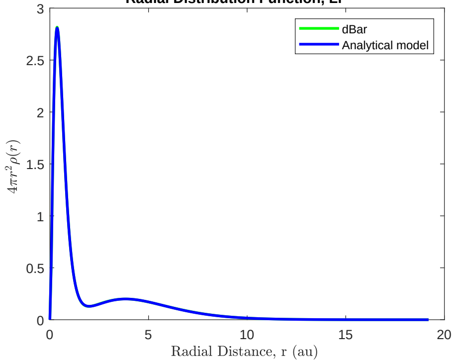
Radial Distribution Function, Li exc1
