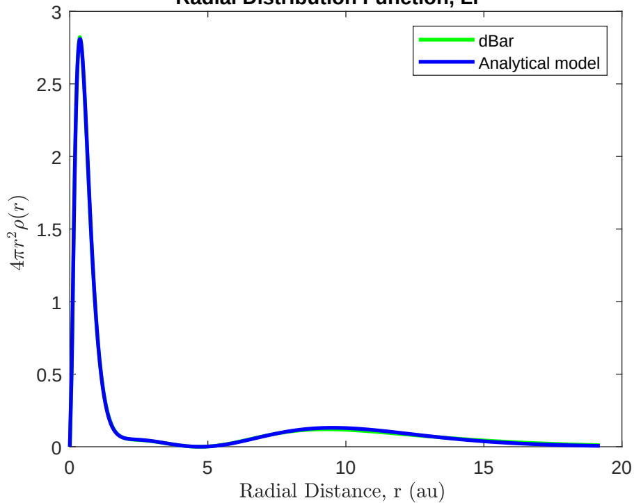
Radial Distribution Function, \text{Li}^{\text{exc}2}
