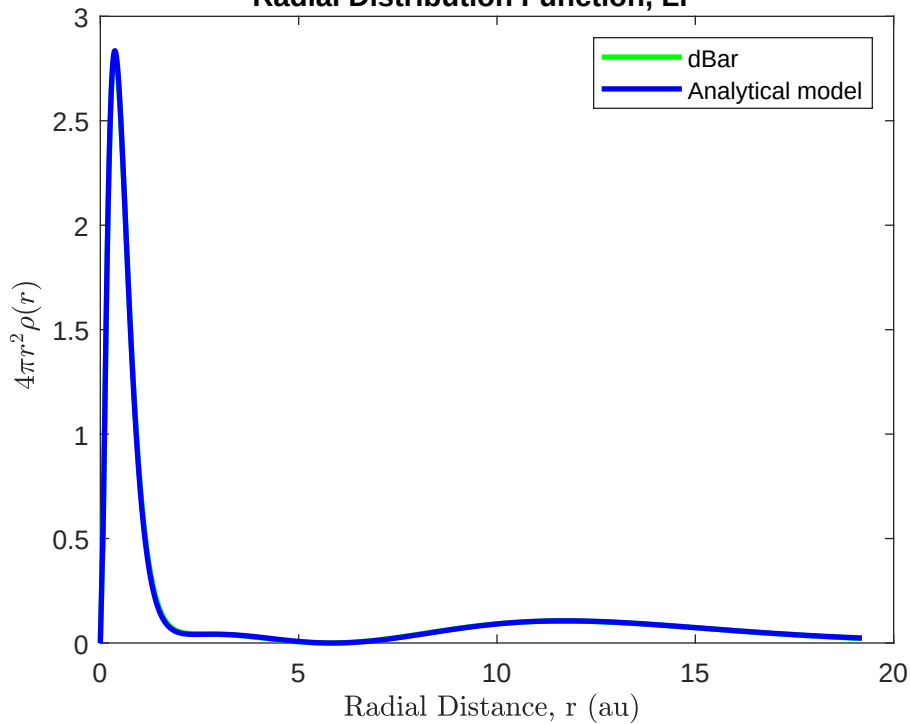
Radial Distribution Function, Li exc3
