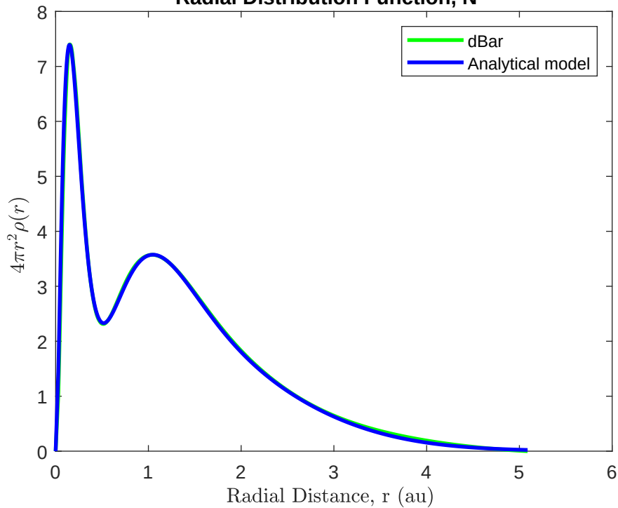
Radial Distribution Function, N^{-1}
