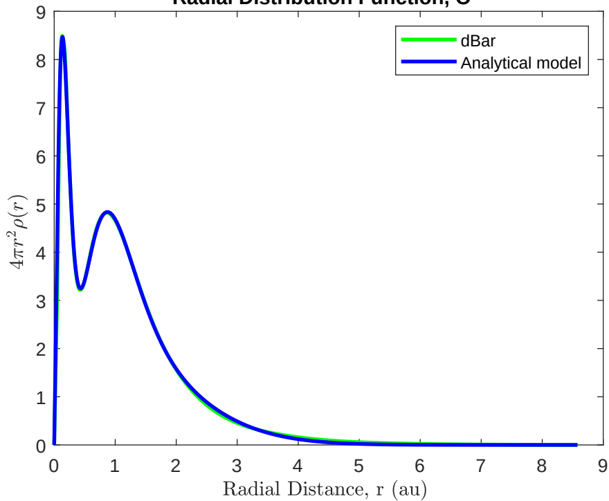
Radial Distribution Function, O^{-1}
