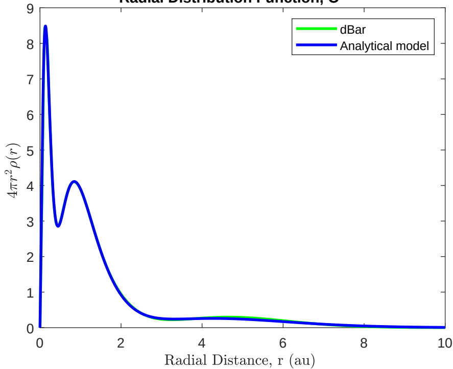
Radial Distribution Function, O^{\text{exc2}}
