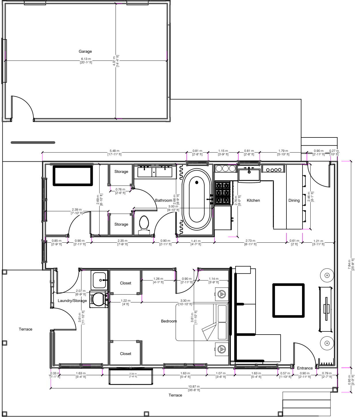
DIMENSIONAL FLOOR PLAN
