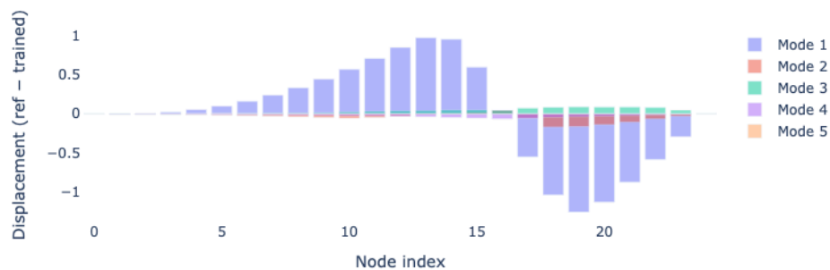
Nodal displacement per mode (r-adaptivity)
