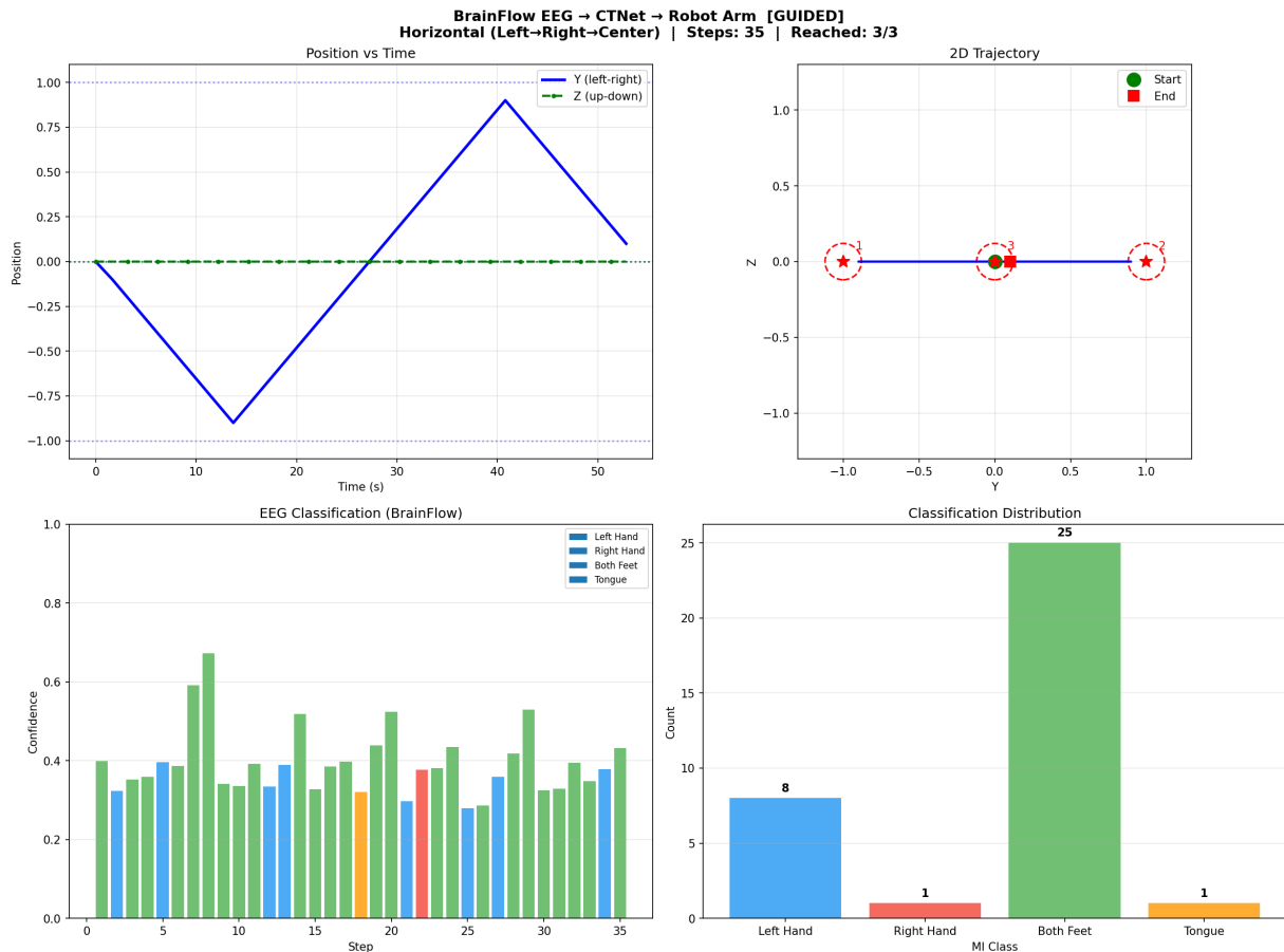
Figure 10: Guided BrainFlow-to-CTNet-to-robot software-interface validation for a horizontal left–right–centre trajectory. The plot records position over time, the 2D path, classifier confidence traces, and the command distribution for a successful guided run.
