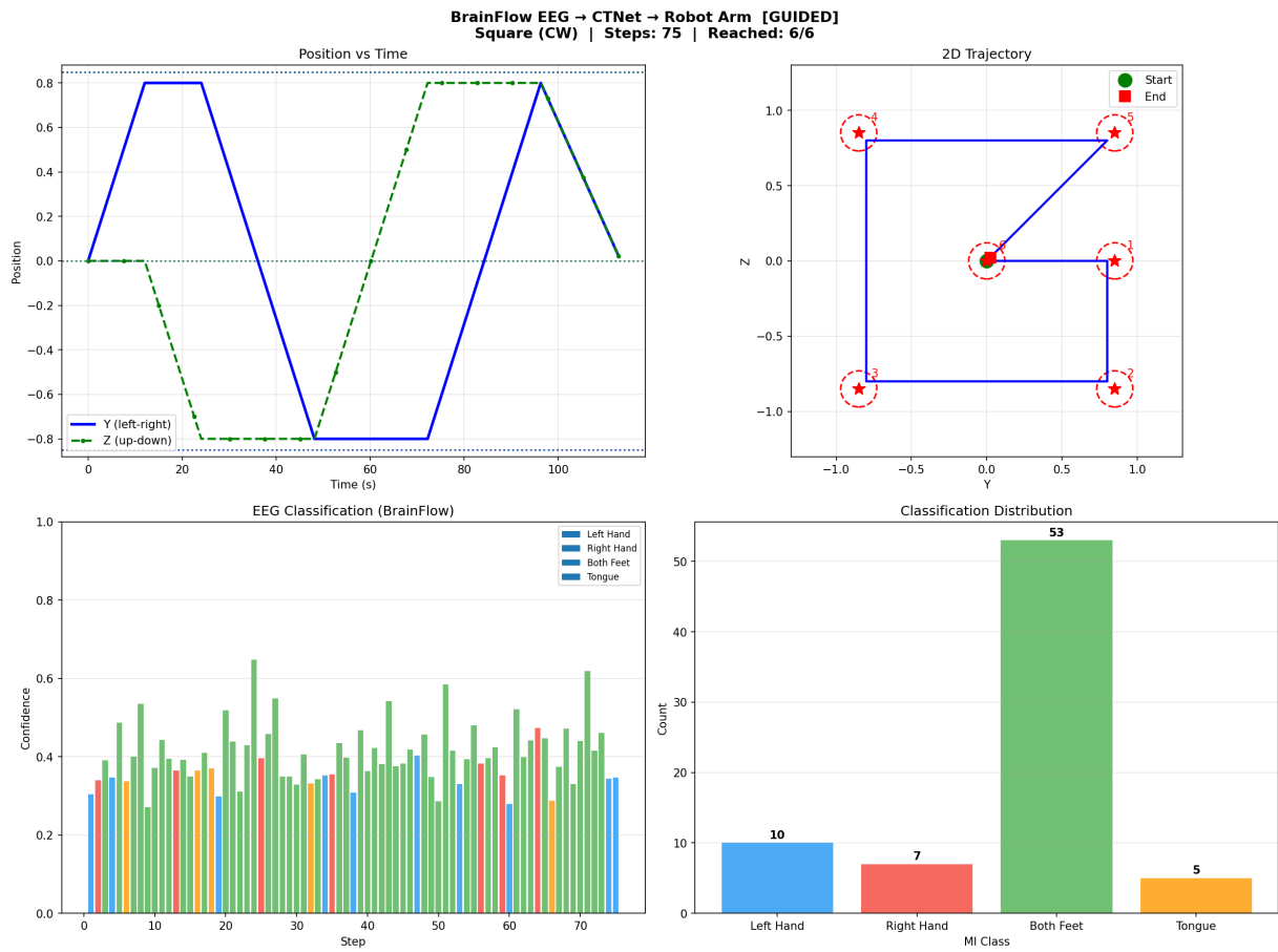
Figure 11: Guided BrainFlow-to-CTNet-to-robot software-interface validation for a clock-wise square trajectory. This figure is included as engineering evidence for the acquisition/classifier/control interface only; it does not represent live human EEG validation.
