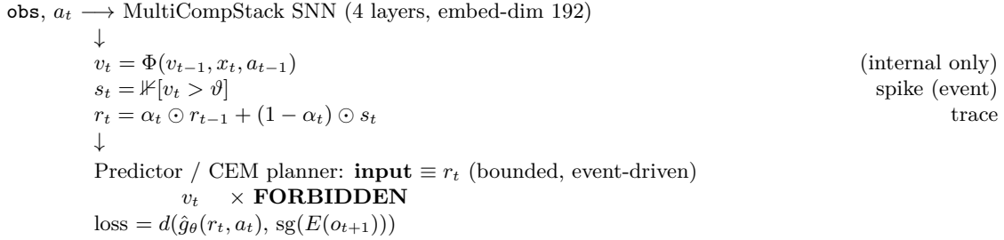
Figure 1 — Membrane-forbidden predictive-state interface
