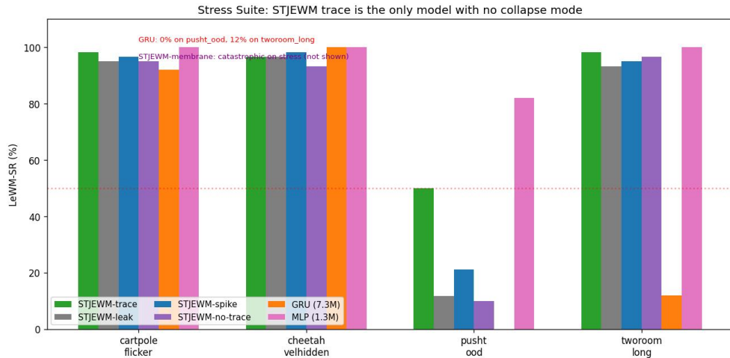
Figure 3: 4-task unsaturated stress suite (3 seeds each). STJEW-trace 96–98% on 3/4 tasks.
