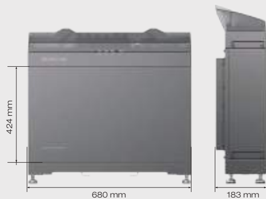
EcoFlow PowerOcean LFP Battery
