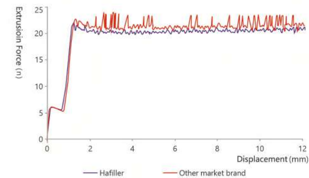
Extrusion Force
