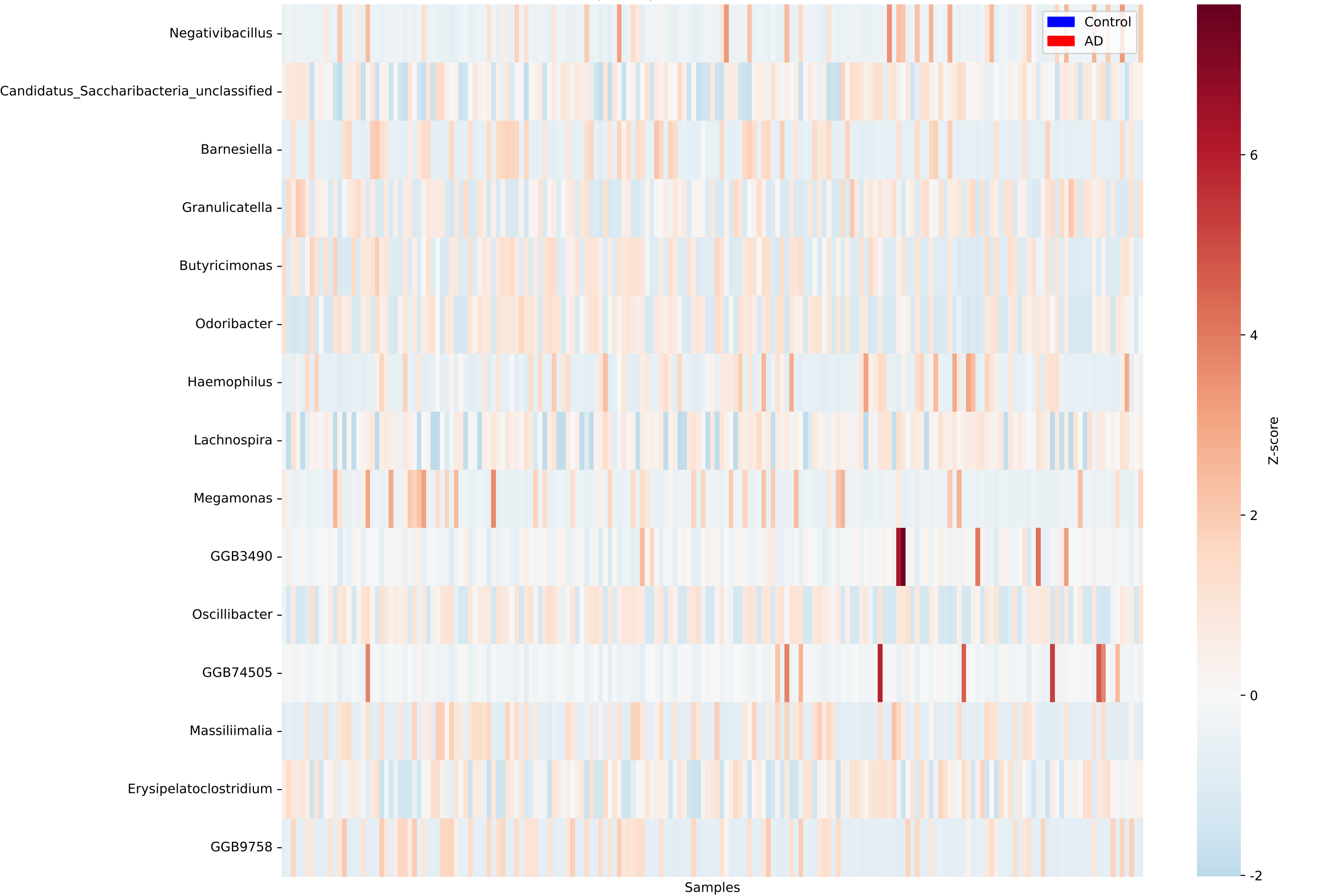
Heatmap of Top 15 Biomarkers (Genus Level)
