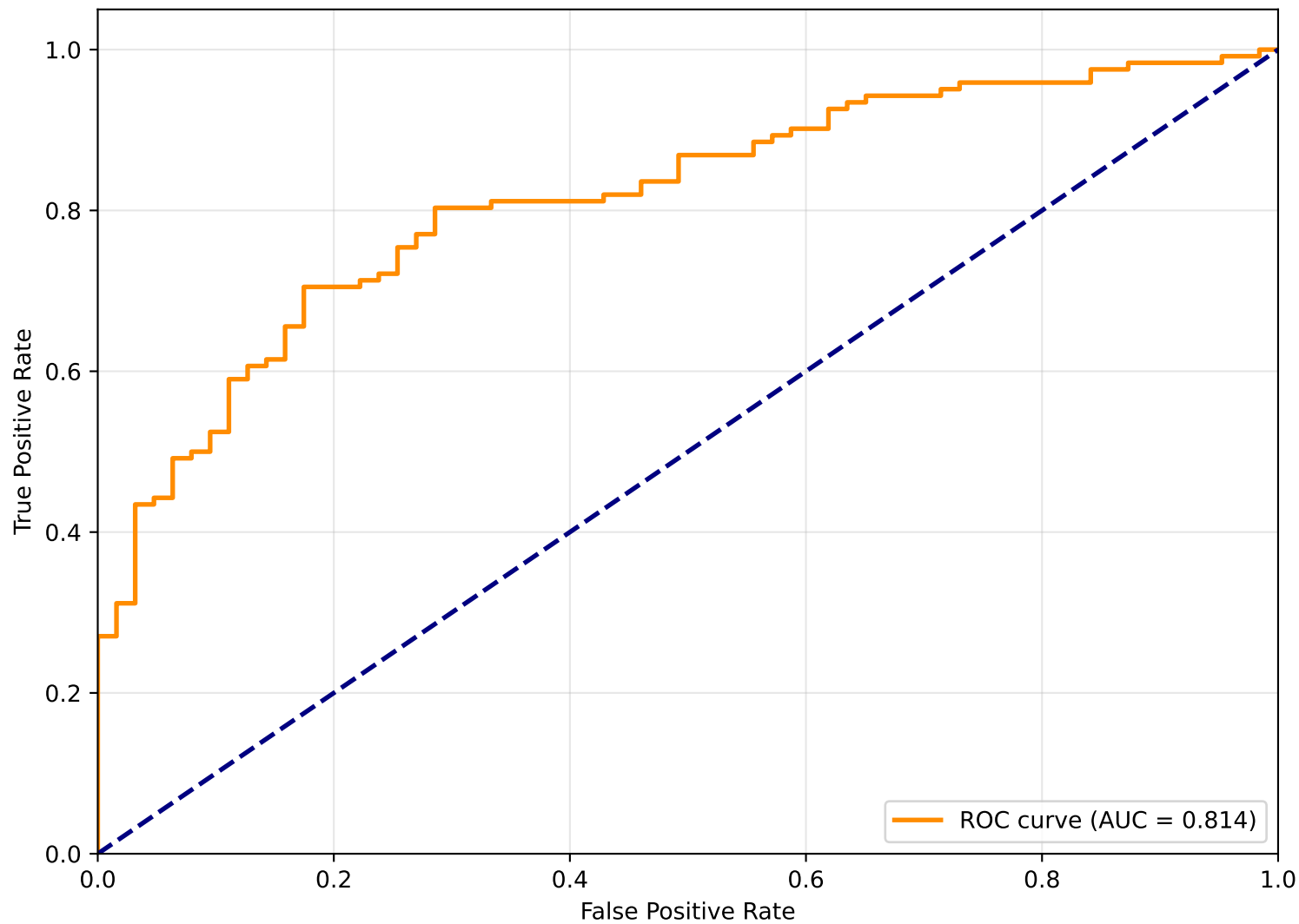
ROC Curve (Genus Level)
