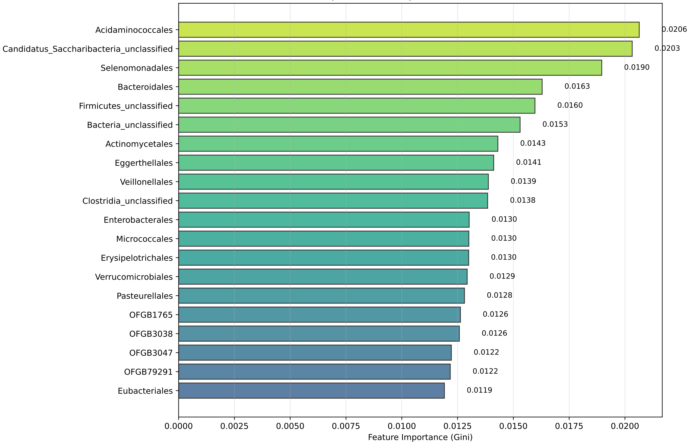
Top 20 Feature Importance (Order Level)
