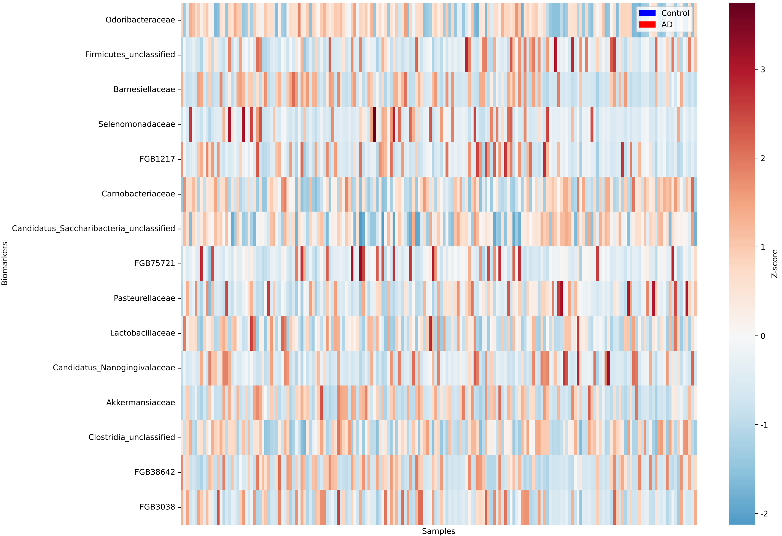
Heatmap of Top 15 Biomarkers (Family Level)
