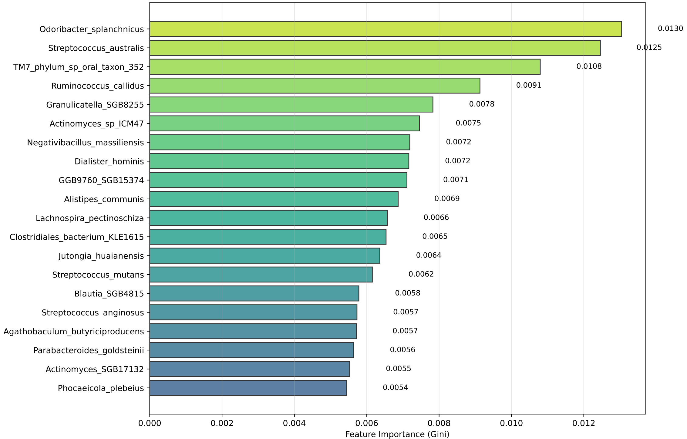
Top 20 Feature Importance (Species Level)
