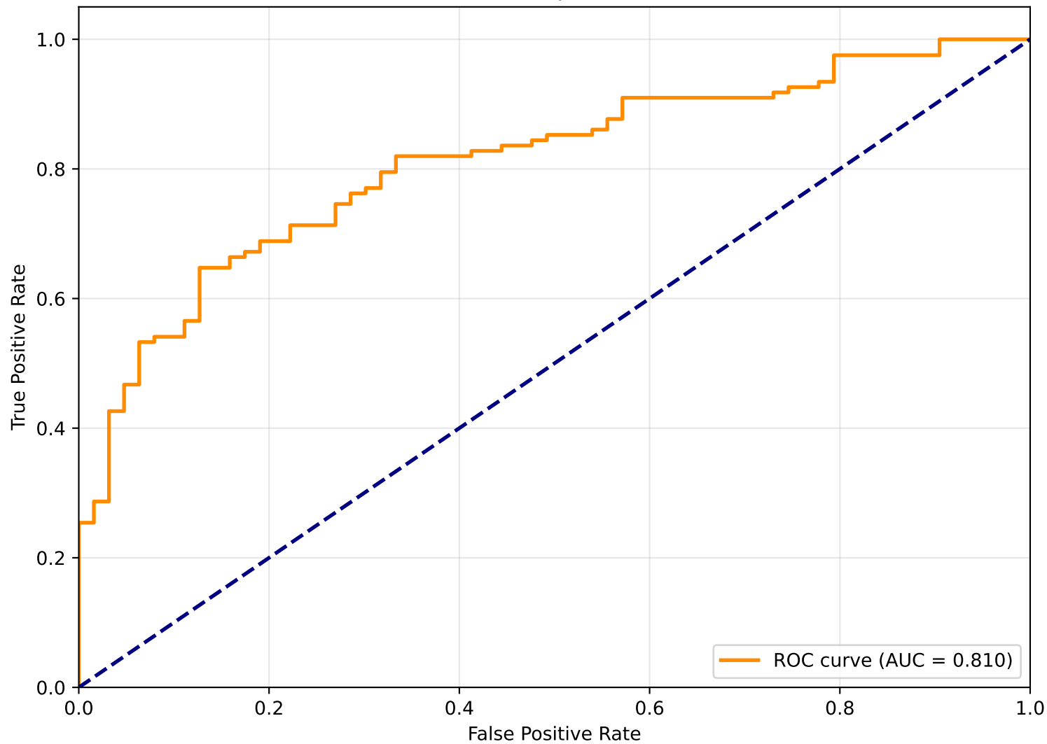
ROC Curve (Species Level)
