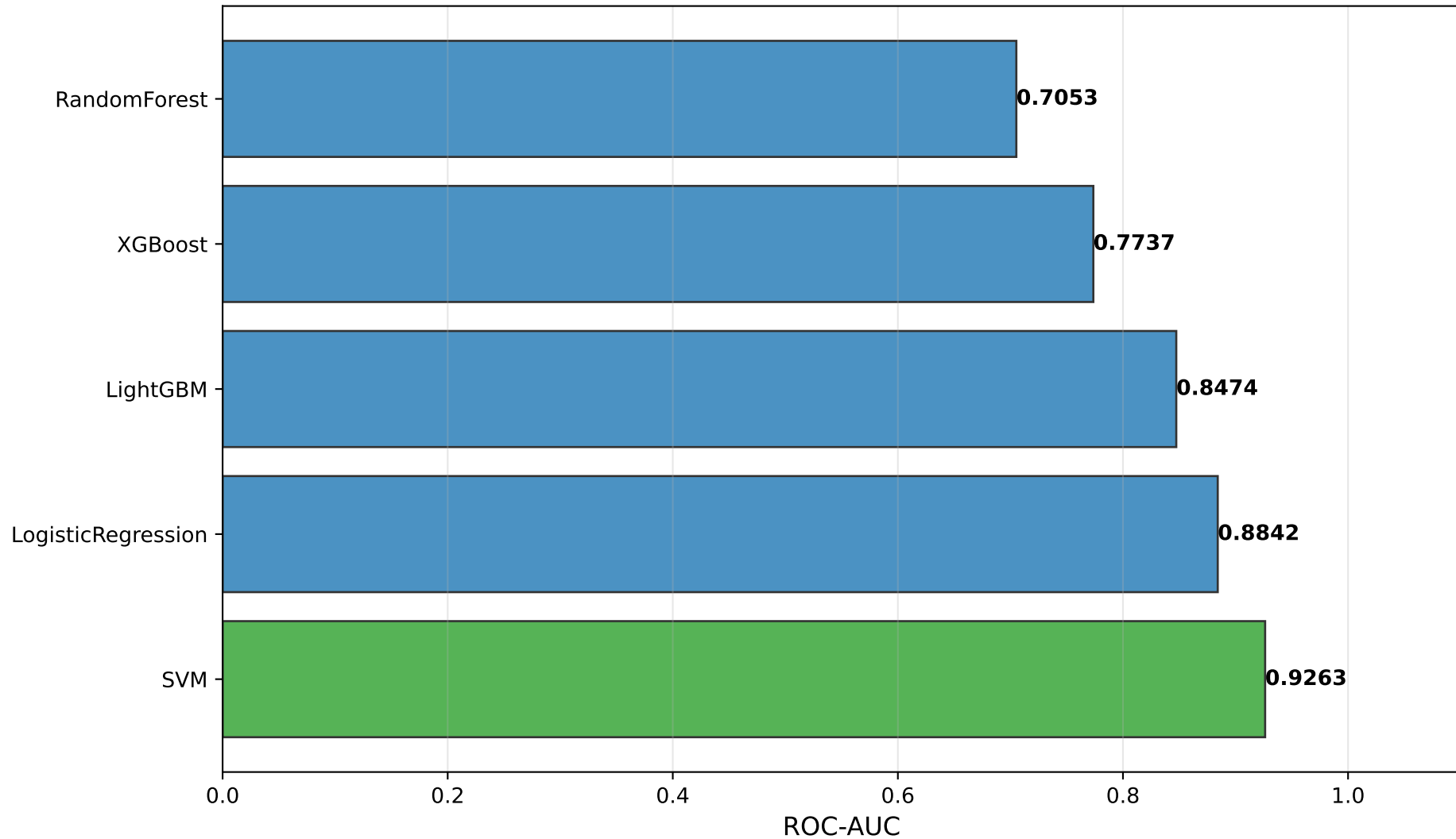
Model Ranking by ROC-AUC
