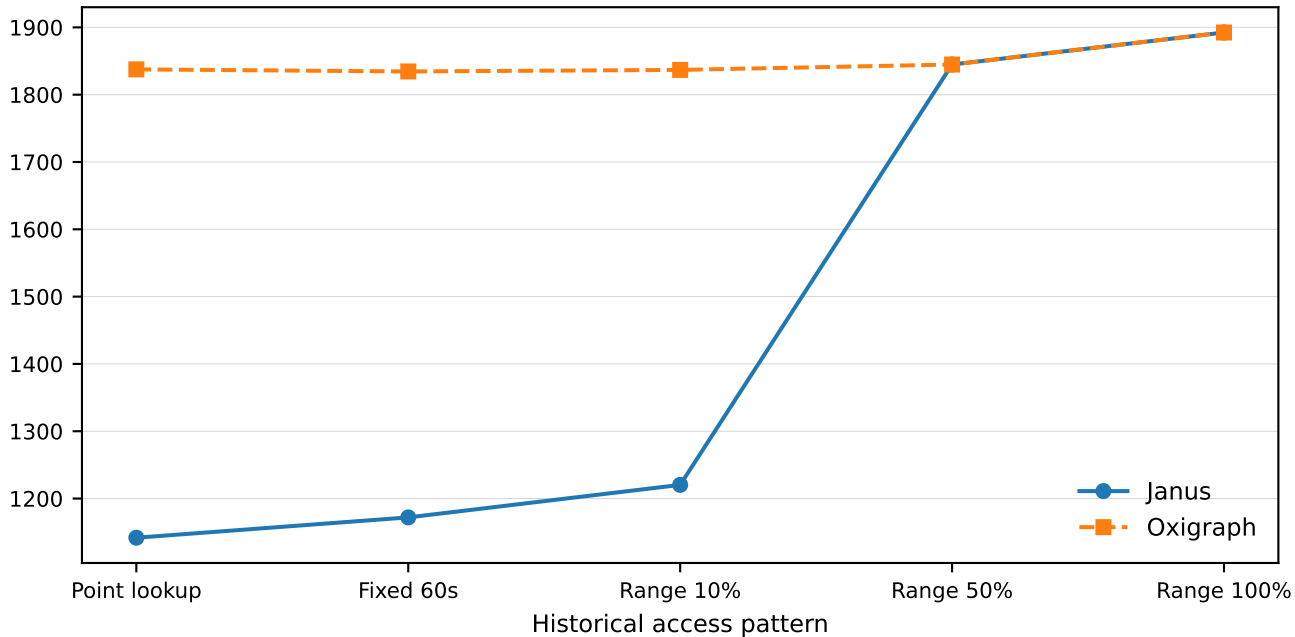
Median peak memory (MB)
