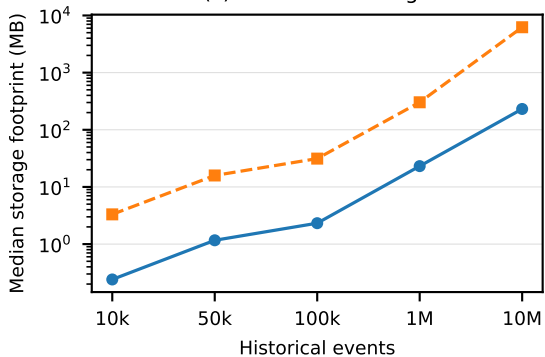
(c) Persistent storage
