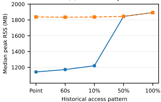
(a) Peak memory
