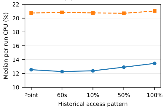
(b) CPU utilization
