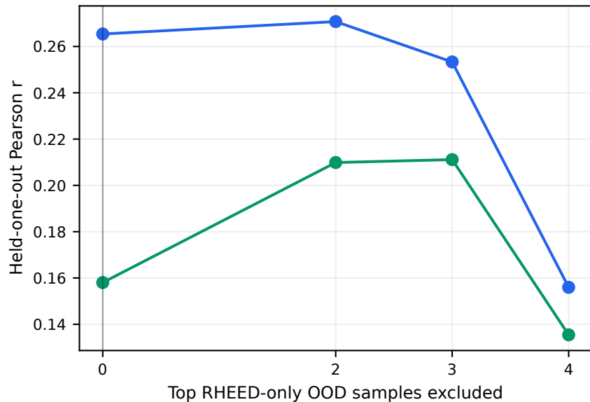
Sensitivity analysis: exclusion does not improve the frozen M12a head
