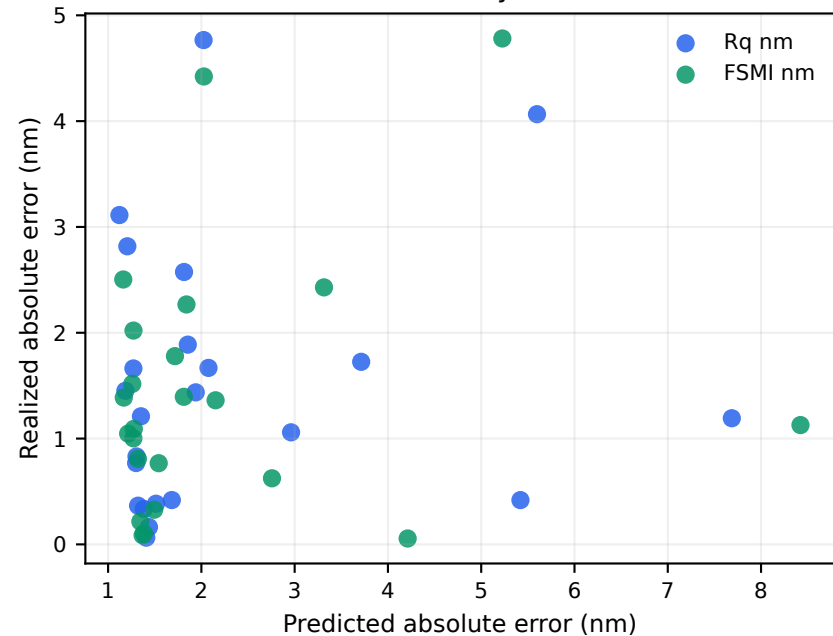
Nested uncertainty calibration
