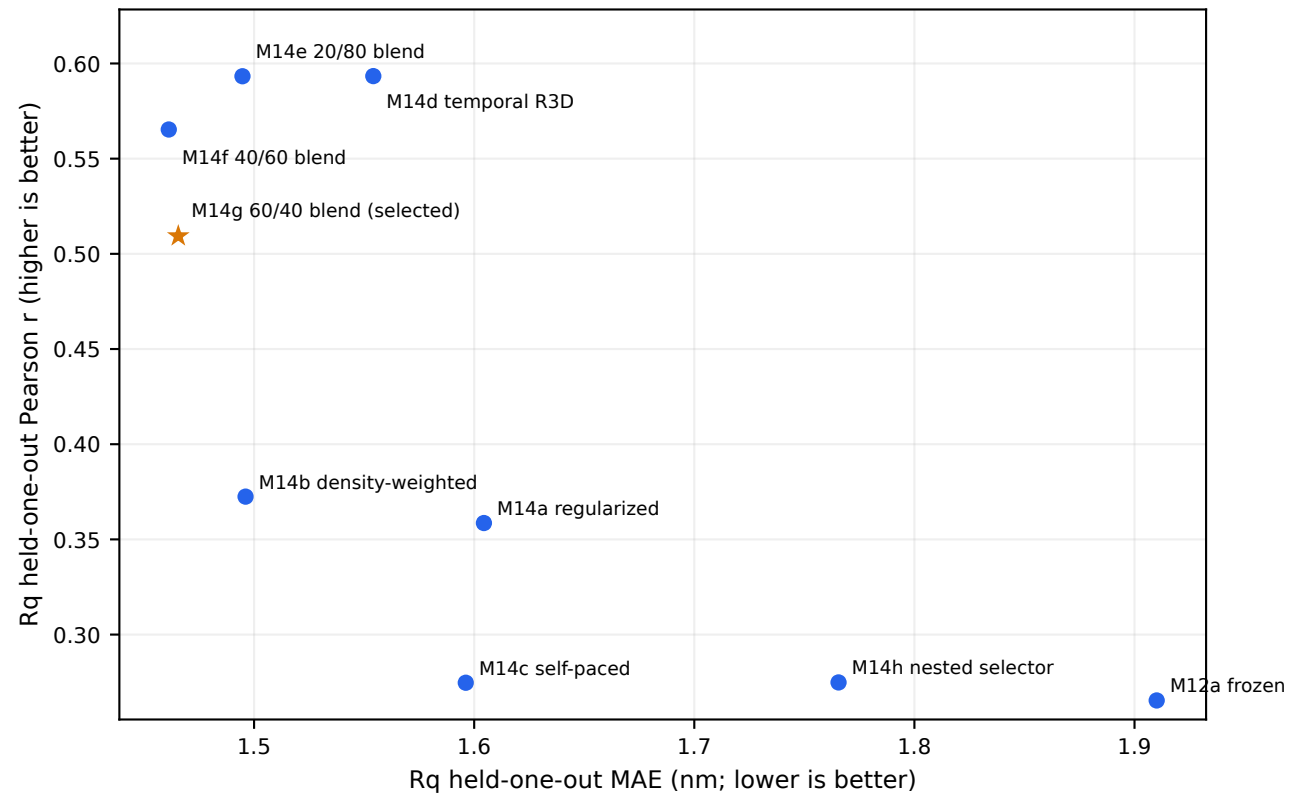
Robust small-sample condition-head ablation
