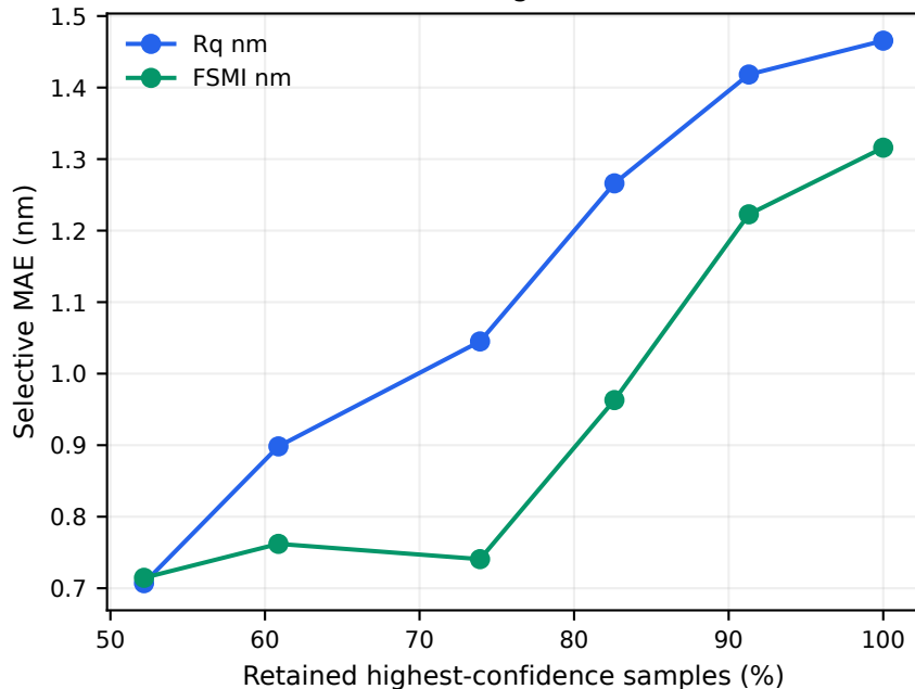
Risk-coverage behavior
