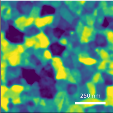
generated AFM Rq=3.54 nm, FSMI=2.16 nm, C=93/100
