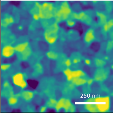
generated AFM Rq=3.00 nm, FSMI=2.81 nm, C=93/100
