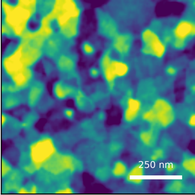
generated AFM Rq=2.61 nm, FSMI=1.89 nm, C=100/100
