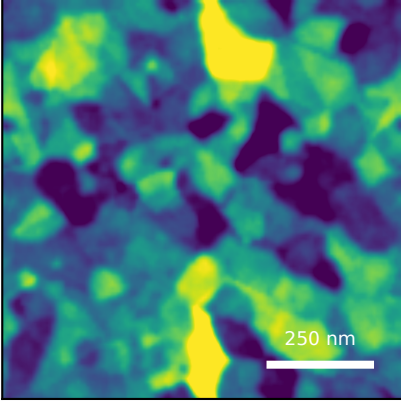
generated AFM Rq=3.23 nm, FSMI=3.64 nm, C=72/100
