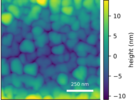
measured AFM Rq=5.34 nm, FSMI=4.21 nm
