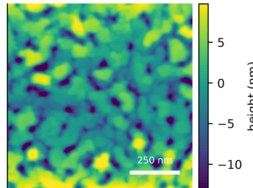
measured AFM
