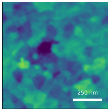
M10 baseline predicted Rq=4.64 nm
