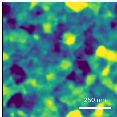
M10 baseline predicted Rq=2.62 nm
