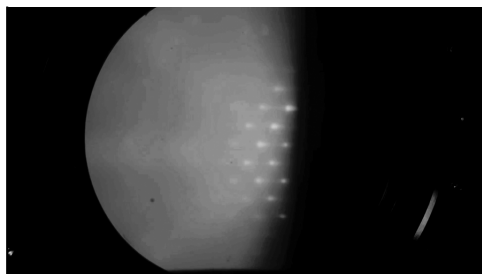
6090 RHEED key frame
