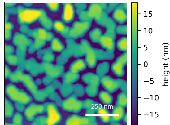
measured AFM Rq=5.87 nm, FSMI=4.88 nm
