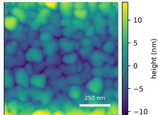
measured AFM Rq=4.69 nm, FSMI=3.17 nm
