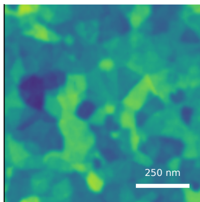
generated AFM Rq=3.01 nm, FSMI=1.79 nm, C=65/100
