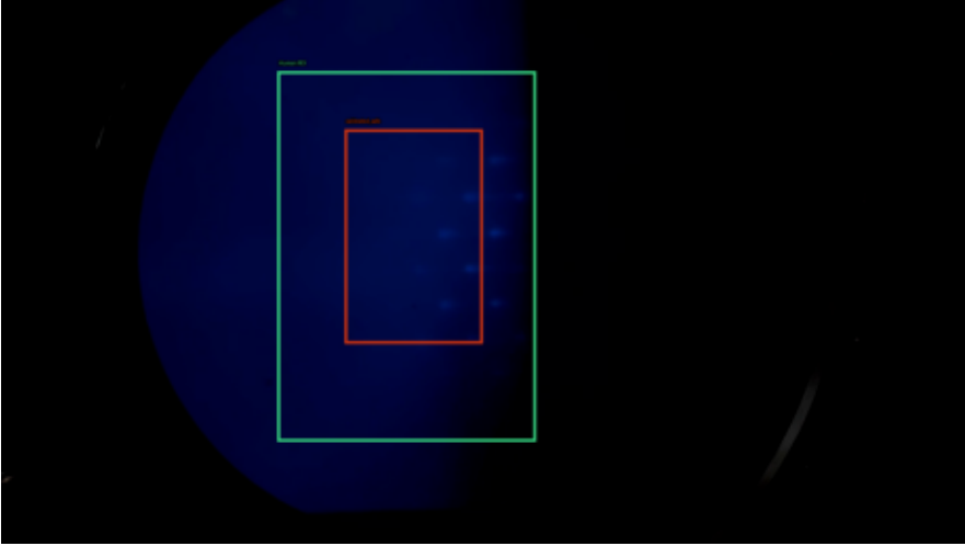
6087 | IoU 0.59 | safe 99.8%
