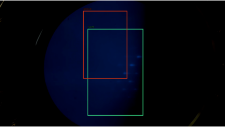
6055 | IoU 0.53 | safe 99.8%
