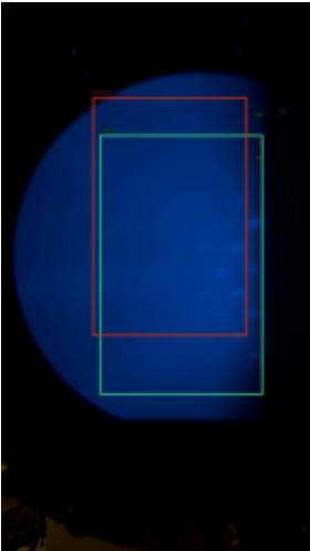
6033 | IoU 0.60 | safe 99.8%
