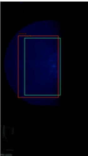
6028 | IoU 0.57 | safe 99.8%
