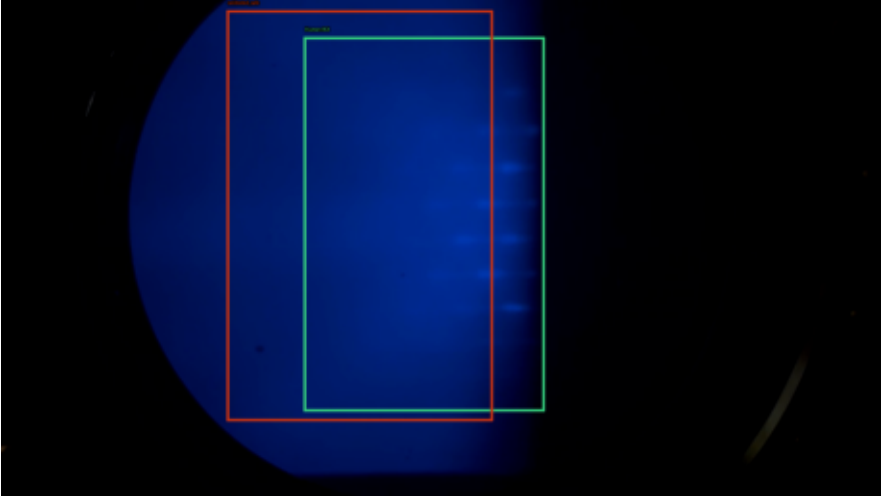
6078 | IoU 0.60 | safe 99.8%
