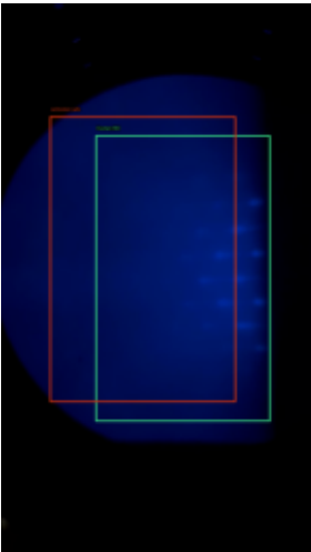
6029 | IoU 0.77 | safe 99.8%
