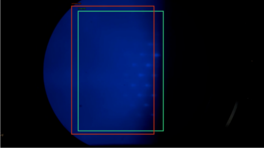
6094 | IoU 0.72 | safe 99.8%
