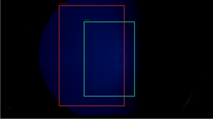
6062 | IoU 0.41 | safe 99.8%
