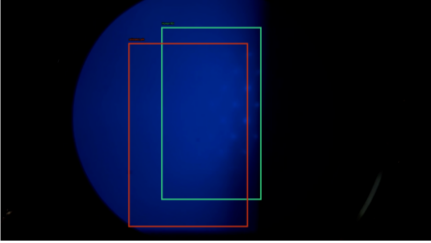
6081 | IoU 0.53 | safe 99.8%
