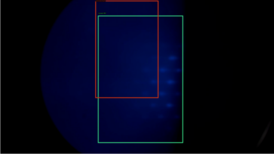
6057 | IoU 0.74 | safe 99.8%
