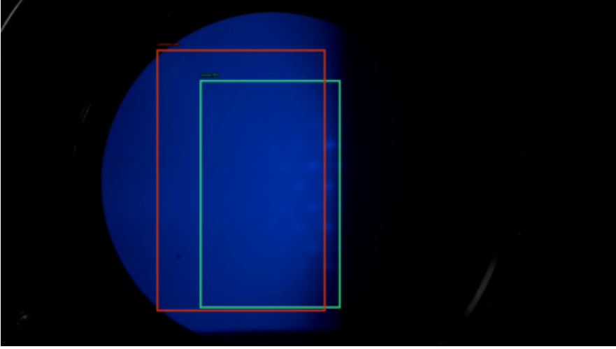
6080 | IoU 0.55 | safe 99.8%
