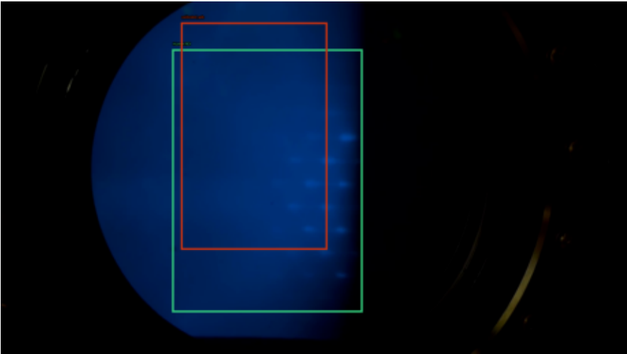
6084 | IoU 0.62 | safe 99.8%
