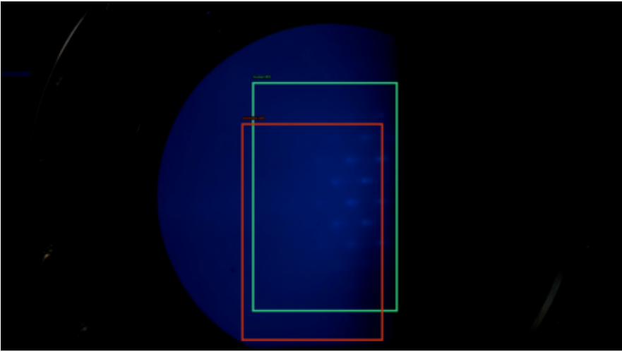
6085 | IoU 0.31 | safe 99.8%
