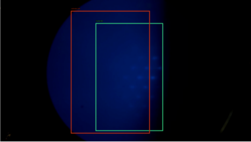
6056 | IoU 0.42 | safe 99.8%
