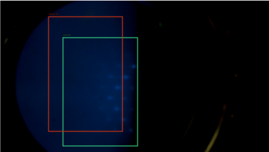
6070 | IoU 0.38 | safe 99.8%
