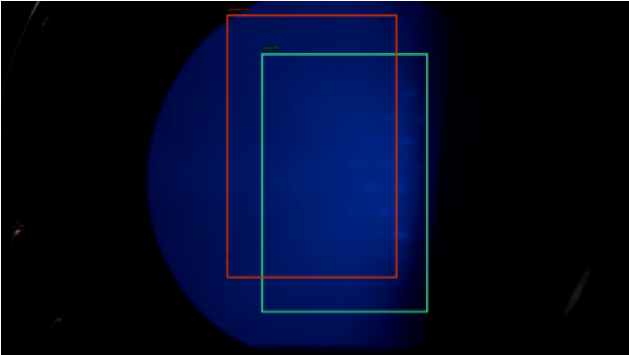
6048 | IoU 0.34 | safe 99.8%
