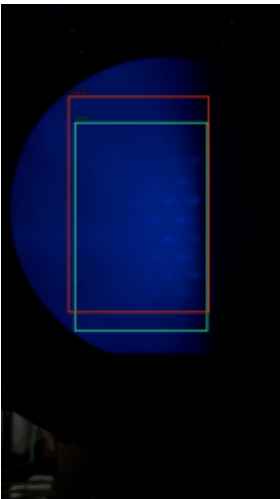
6029 | IoU 0.77 | safe 99.8%
