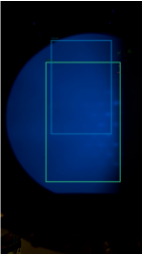
6043 | IoU 0.36 | safe 99.8%
