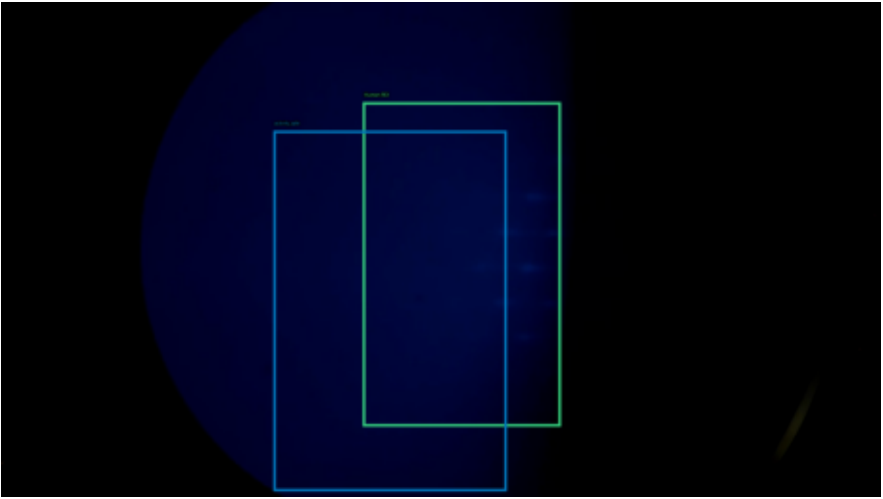
6072 | IoU 0.56 | safe 99.8%
