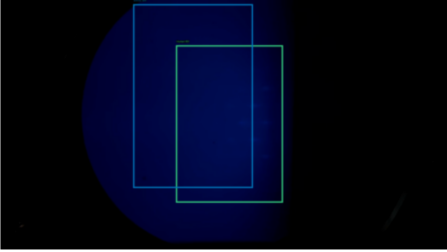
6062 | IoU 0.39 | safe 99.8%
