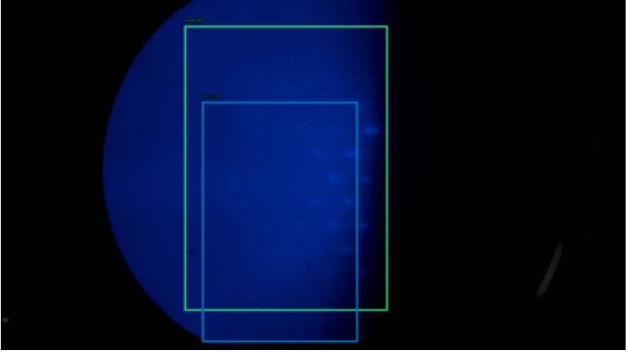
6094 | IoU 0.49 | safe 99.8%
