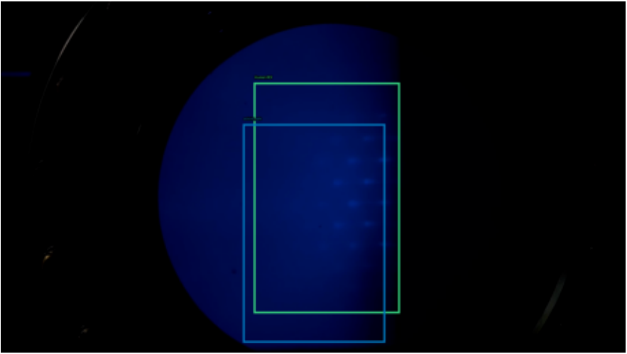
6085 | IoU 0.31 | safe 99.8%
