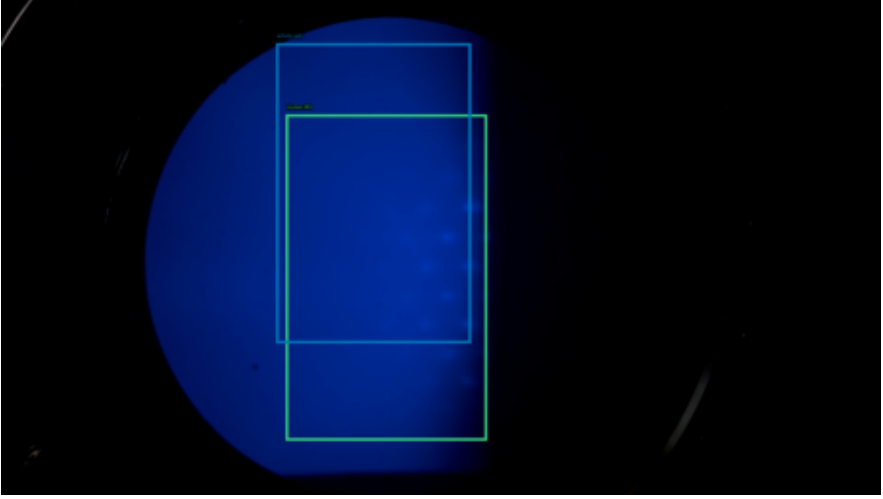
6080 | IoU 0.41 | safe 99.9%
