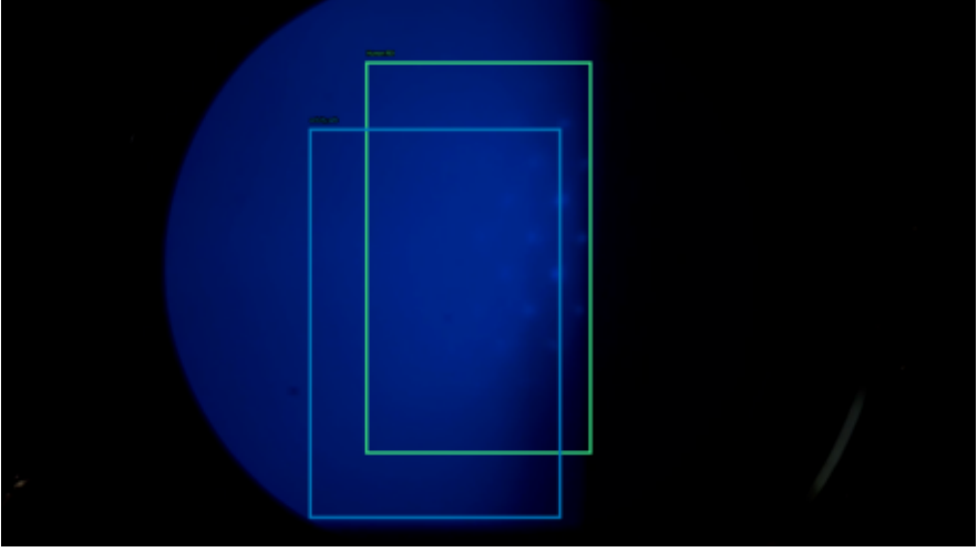
6081 | IoU 0.52 | safe 99.8%
