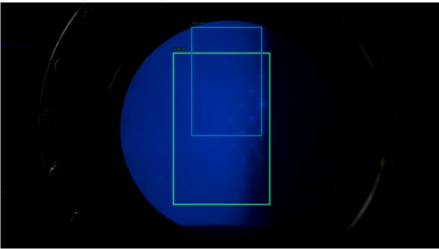
6043 | IoU 0.36 | safe 99.8%
