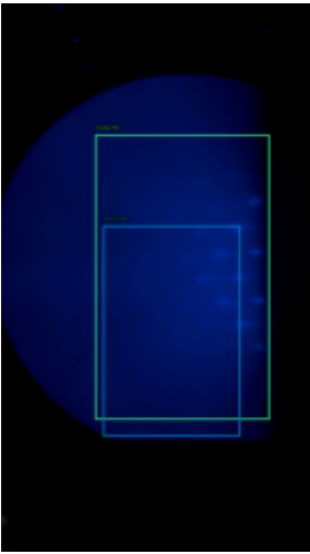
6029 | IoU 0.58 | safe 99.8%
