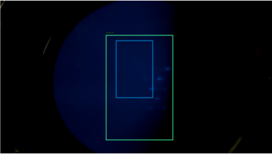
6055 | IoU 0.25 | safe 99.9%
