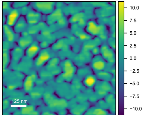
Ground-truth AFM Rq=4.09 nm Ra=3.20 nm
