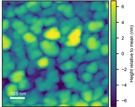
Ground-truth AFM Rq=2.86 nm Ra=2.27 nm
