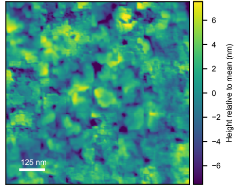
Retrieval-augmented representative AFM Rq=3.06 nm
