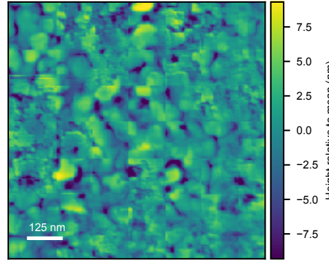
Retrieval-augmented representative AFM Rq=3.39 nm
