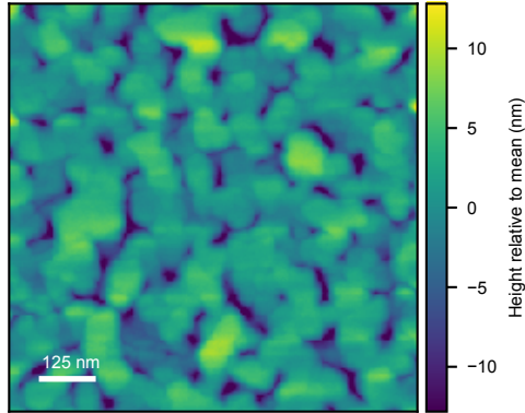
Retrieved real AFM exemplar source=6062 Rq=3.06 nm
