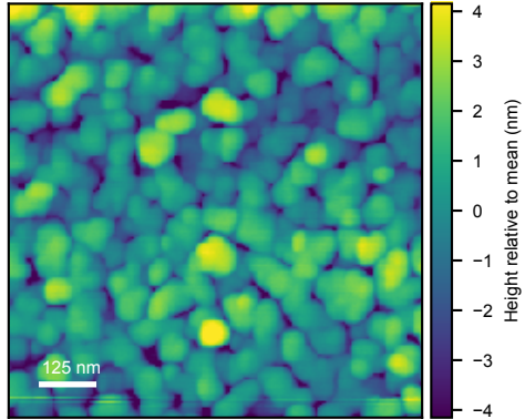
Ground-truth AFM Rq=2.74 nm Ra=2.20 nm
