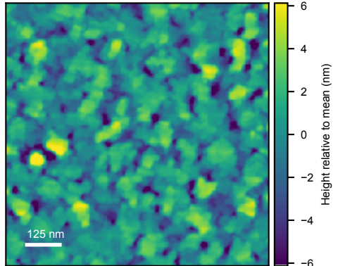
Retrieved real AFM exemplar source=6090 Rq=3.82 nm
