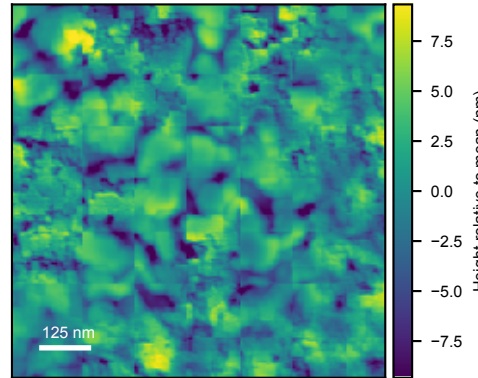
Retrieval-augmented representative AFM Rq=3.82 nm
