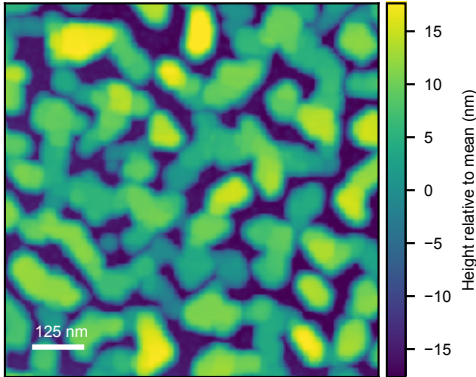
Ground-truth AFM Rq=10.30 nm Ra=9.14 nm
