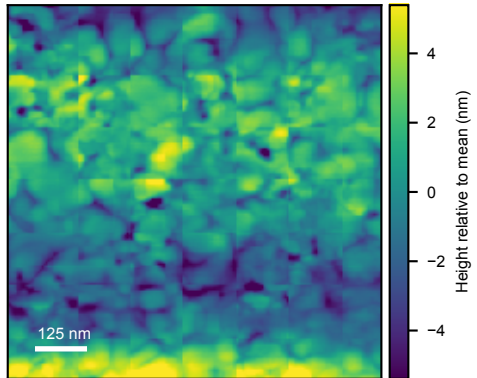
Retrieval-augmented representative AFM Rq=2.25 nm
