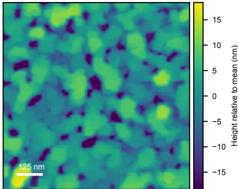
Retrieved real AFM exemplar source=6033 Rq=2.25 nm
