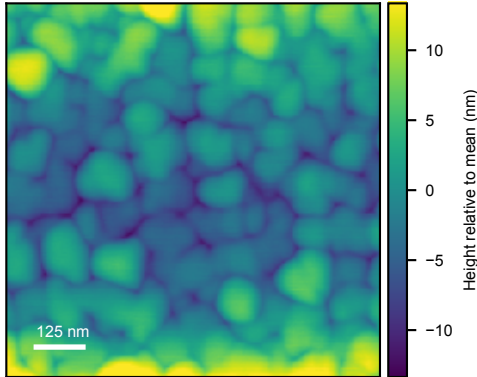
Retrieved real AFM exemplar source=6081 Rq=2.21 nm
