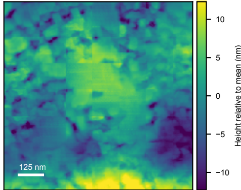
Retrieval-augmented representative AFM Rq=2.21 nm
