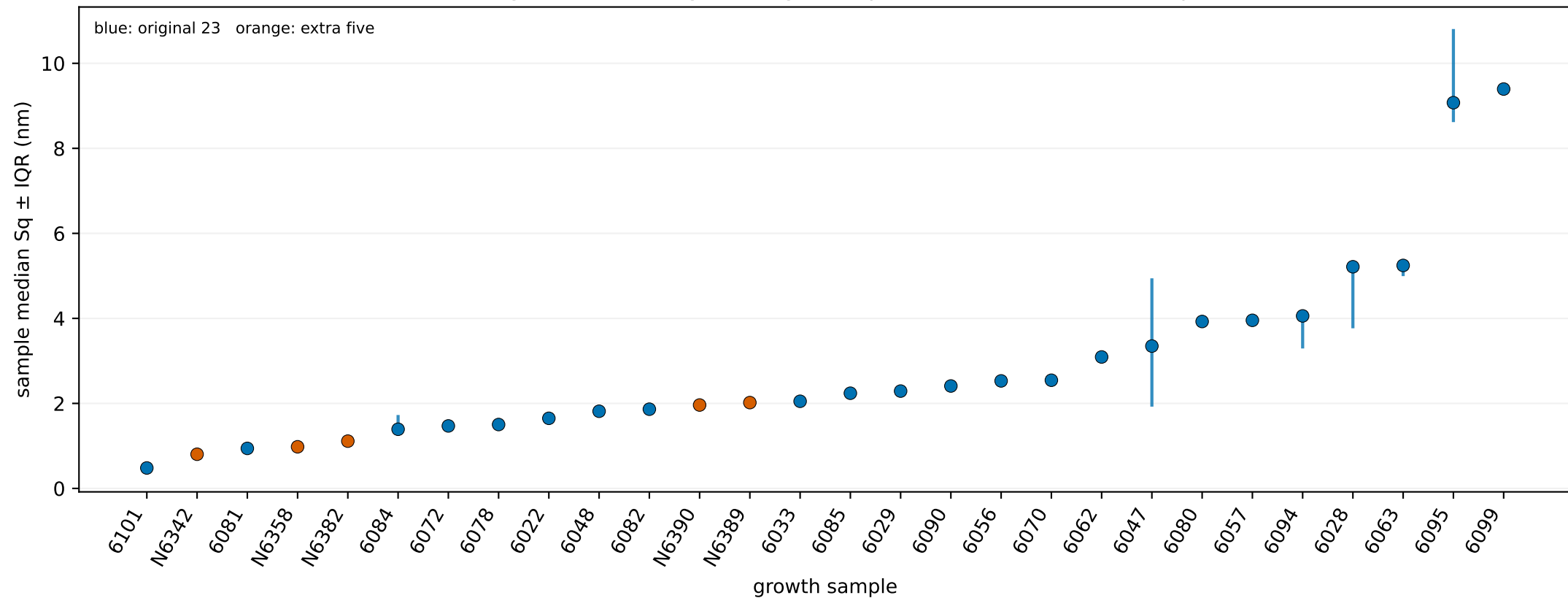
Harmonized 28-growth AFM targets: original 1 \mu\text{m} scans and extra-five 1 \mu\text{m} subfields
