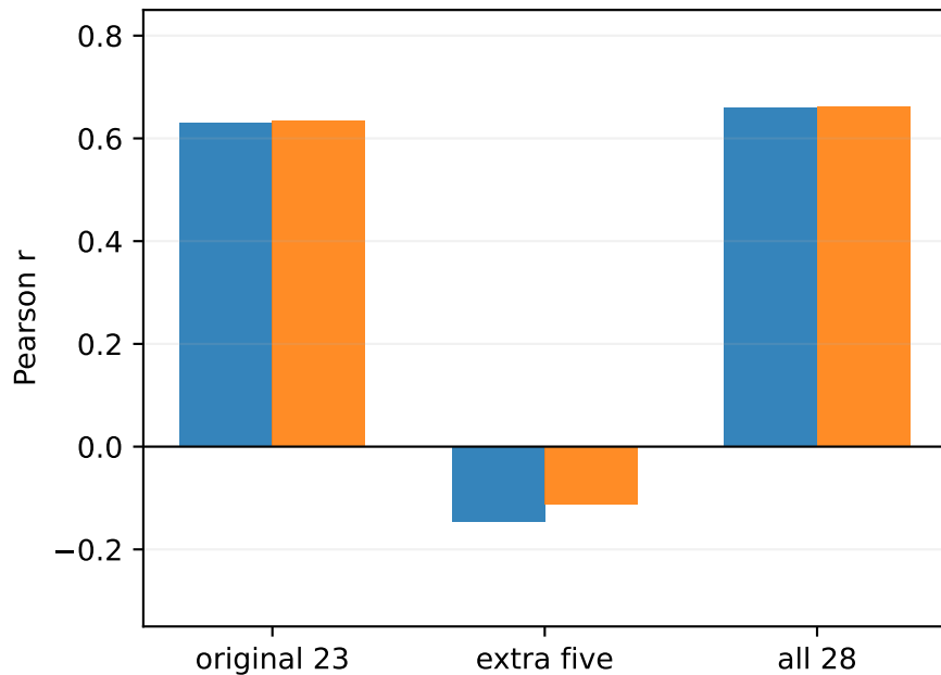
Within-cohort correlation (extra-five range is narrow; n=5)
