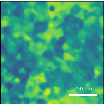
generated AFM predicted Sq=5.05 nm; FSMI=4.30 nm C=10/100
