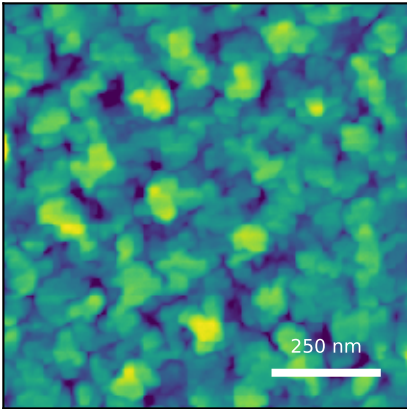
measured AFM displayed scan Sq=2.54 nm sample median Sq=2.54 ± 0.06 nm (IQR)
