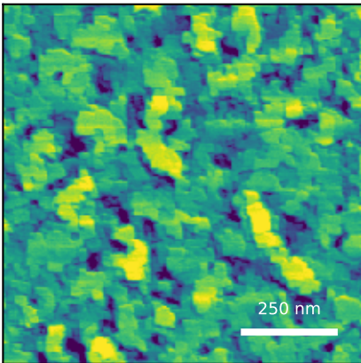
measured AFM displayed scan Sq=9.39 nm sample median Sq=9.39 ± 0.21 nm (IQR)
