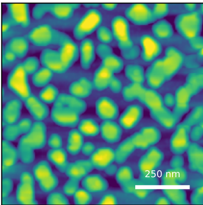
measured AFM displayed scan Sq=9.07 nm sample median Sq=9.07 ± 2.19 nm (IQR)
