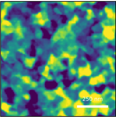
generated AFM predicted Sq=2.74 nm; FSMI=2.25 nm C=41/100
